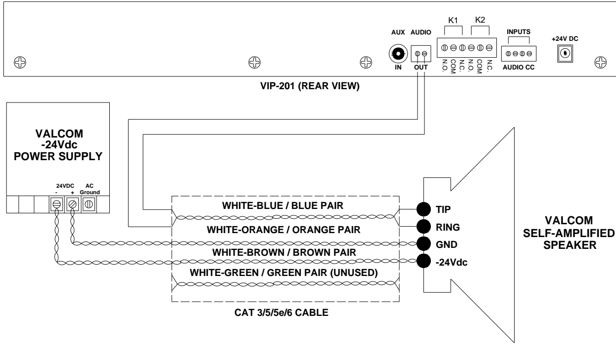
Typical Connection to Valcom Self-amplified Speakers
