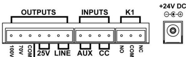
VIP-851-70/100 Rear View
