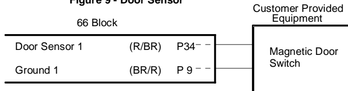
Figure 9 - Door Sensor
