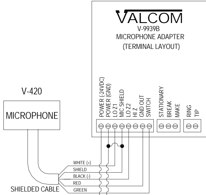
FIGURE 1. CONNECTING ARRANGEMENT
