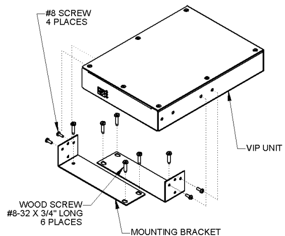
Figure 2. Wall Mount
