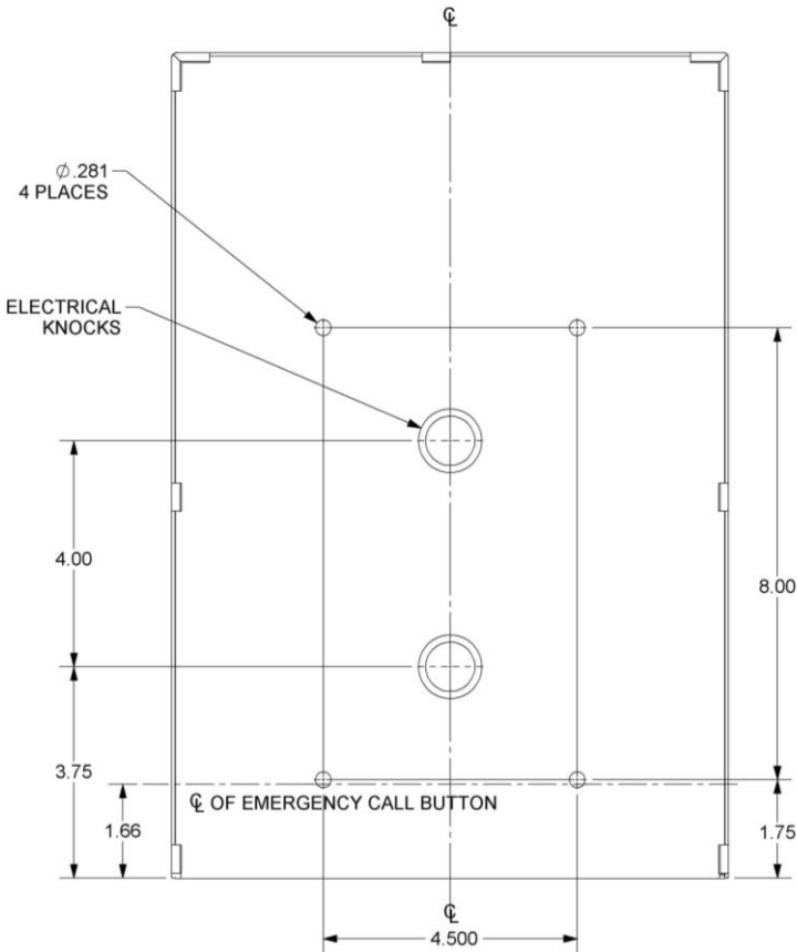
Figure 1. Mounting information
