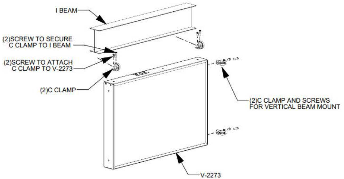
Figure 2: Beam Mounting
