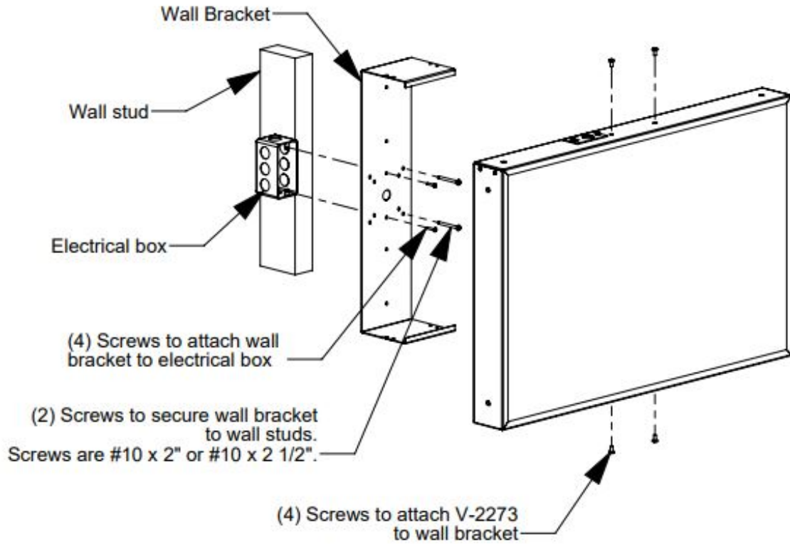
Figure 1: Wall or Surface Mounting
