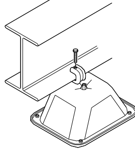
ATTACH FLEXHORN TO BEAM
