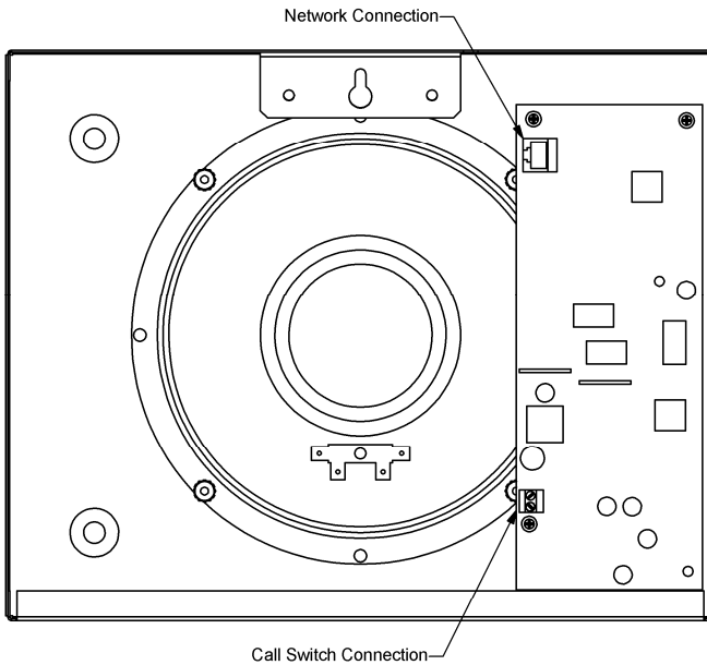
FIG 1. VIP-430 CONNECTIONS
