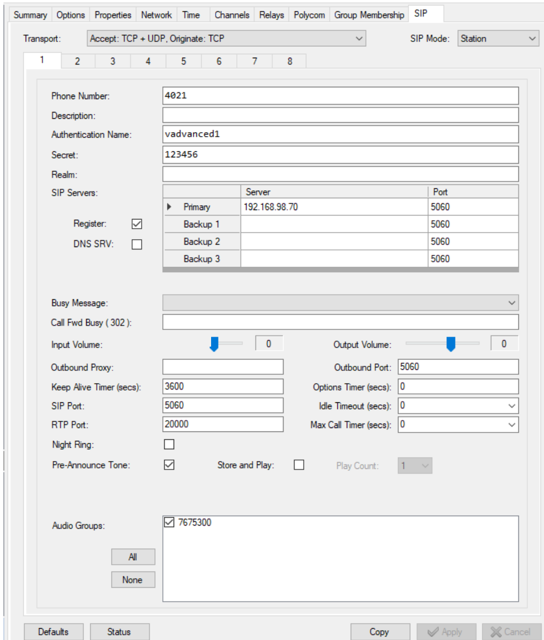
Figure 142: SIP Tab Using SIP Mode Station Dialog Box
