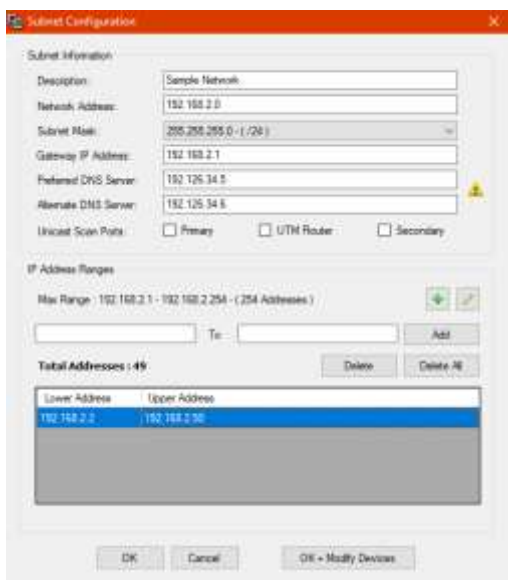
Figure 5: Subnet Configuration Dialog Box
