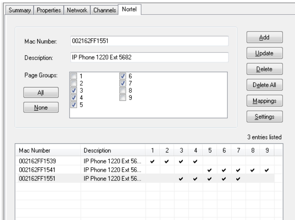
Figure 146: Nortel Tab Dialog Box
