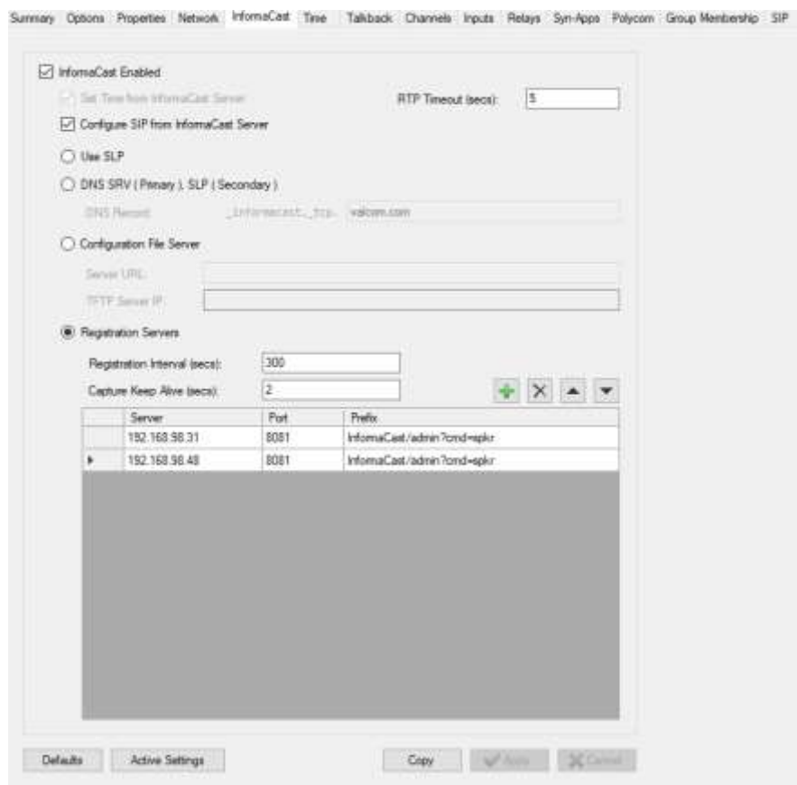
Figure 105: InformaCast Using Registration Servers Option Dialog Box
