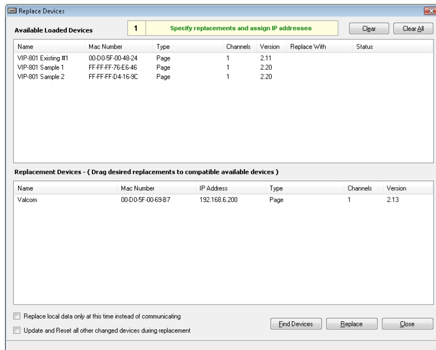
Figure 45: Replace Devices Dialog Box
