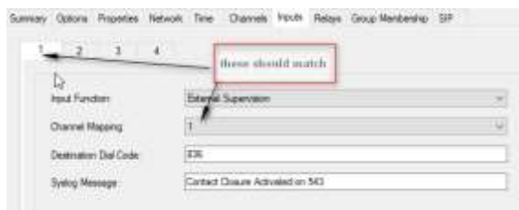
Figure 120: Inputs Tab Using External Supervision Function Dialog Box
