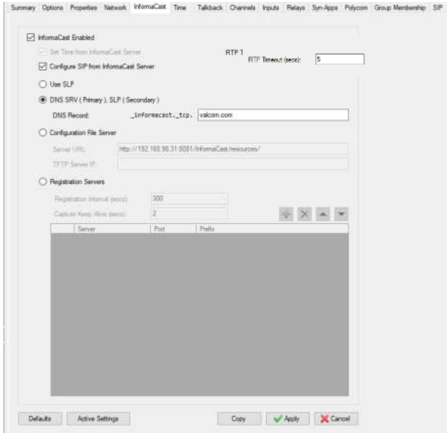
Figure 103: InformaCast Tab Dialog Box
