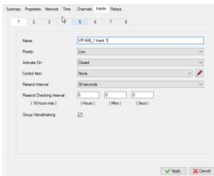
Figure 124: Inputs Tab for VIP-848 Device Dialog Box
