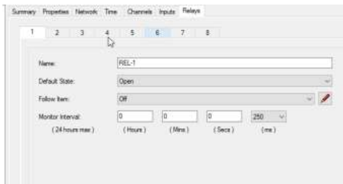
Figure 128: Relays Tab for VIP-848 Dialog Box
