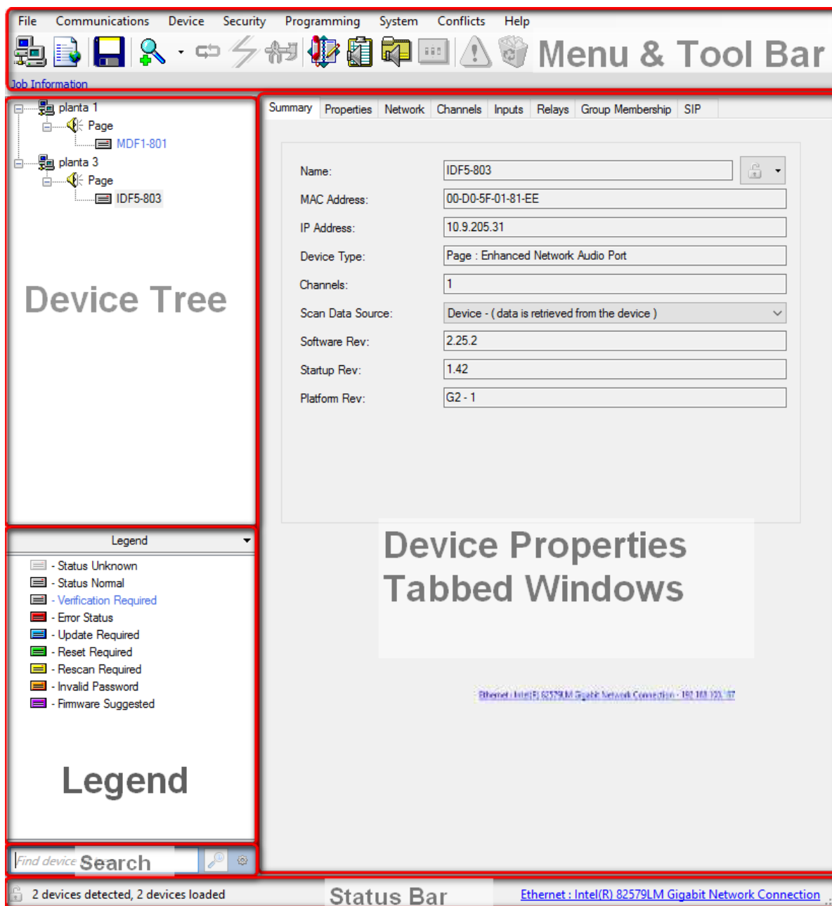
Figure 2: Main Application Dialog Box
