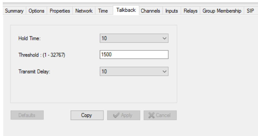
Figure 112: Talkback Tab Dialog Box
